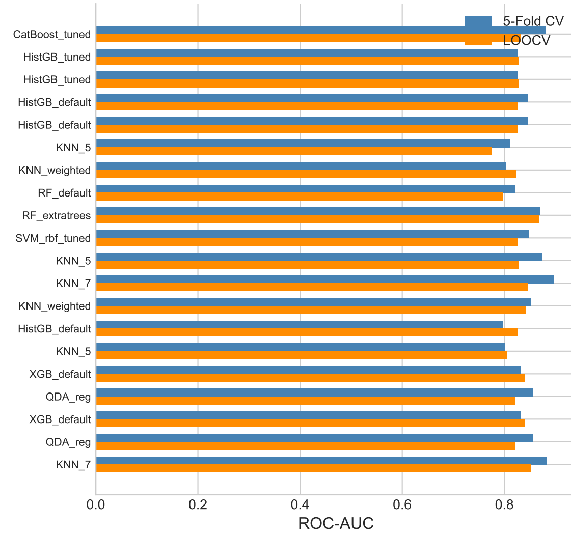
5-Fold CV vs LOOCV ROC-AUC (Two-Class)
