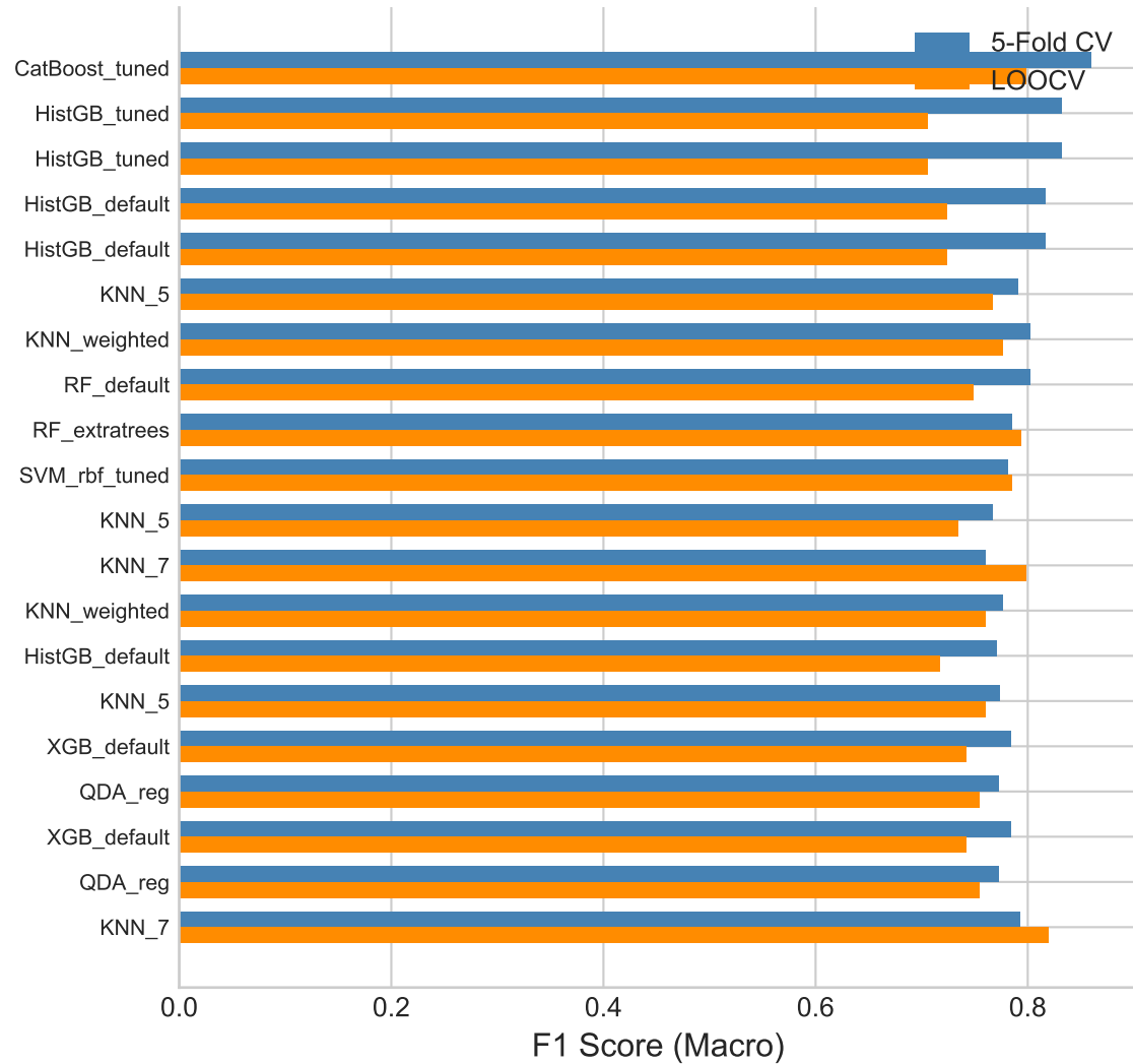
5-Fold CV vs LOOCV F1 Score (Two-Class)
