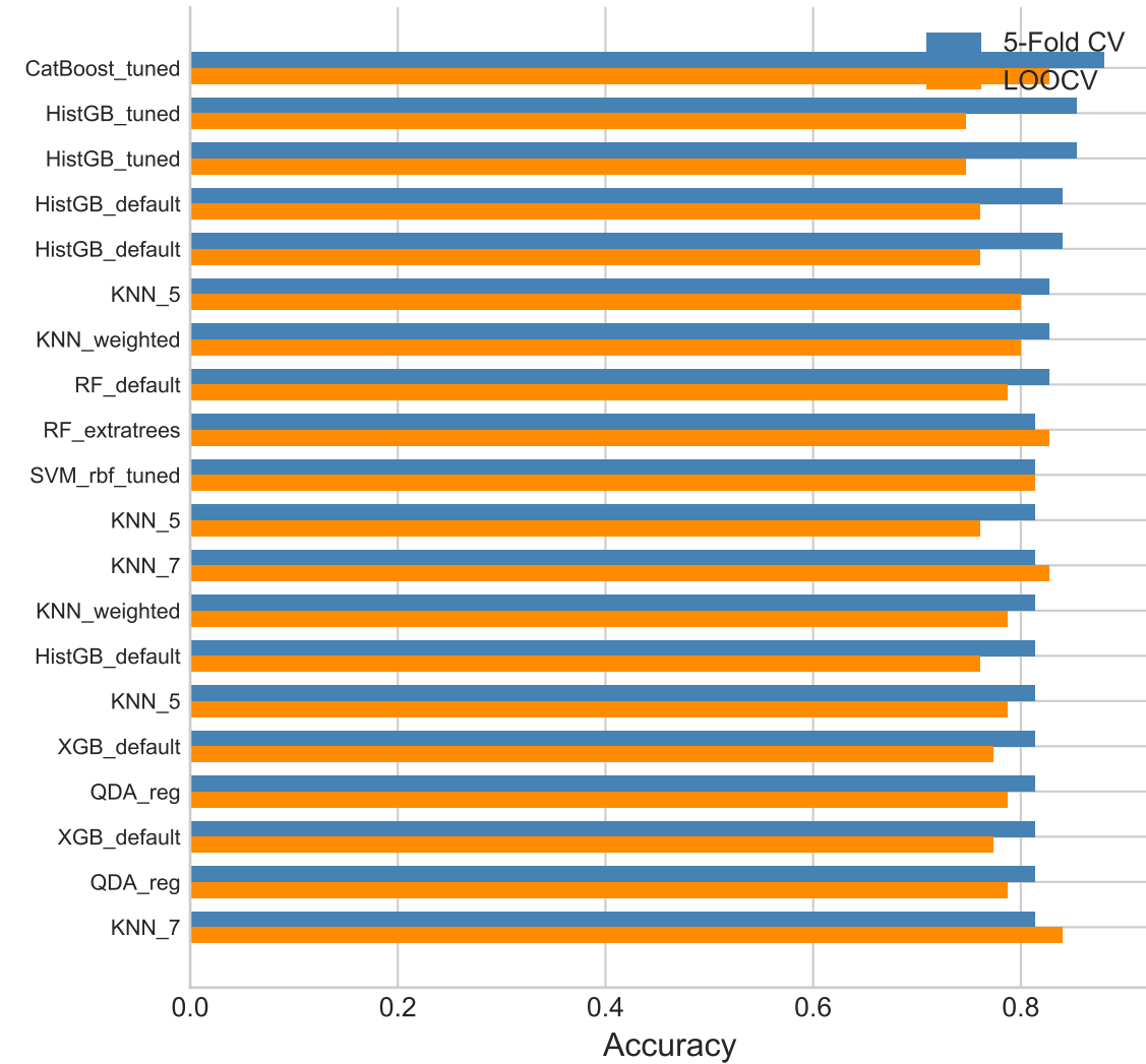
5-Fold CV vs LOOCV Accuracy (Two-Class)
